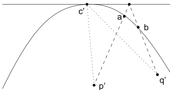
Figure 1: The image of X under \Phi .
