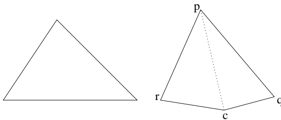
Figure 4: The comparison triangle \tilde{\Delta} pqr and the glued-together quadrilateral Q .
