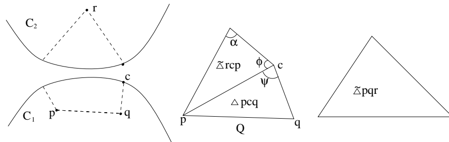
Figure 5: A visual model for \Delta qpr , the quadrilateral Q , and comparison triangle \tilde{\Delta}pqr .
